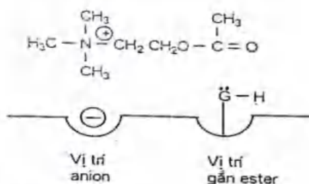
Cholinesterase
