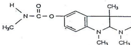
Physostigmin
