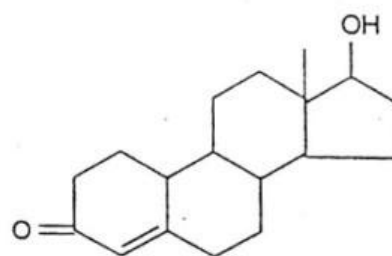
19 nortestosteron
